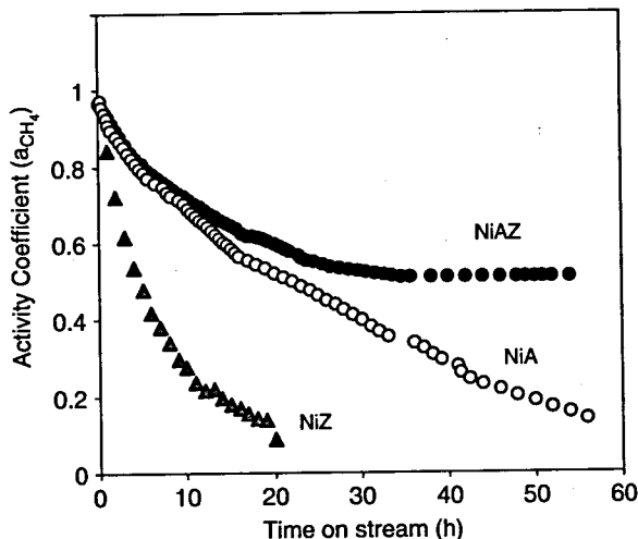
Fig. 3. Deactivation tests of the studied catalysts at 700^\circ C (NiA (o), NiAZ (●), NiZ (▲)). For the conditions, see the text.
