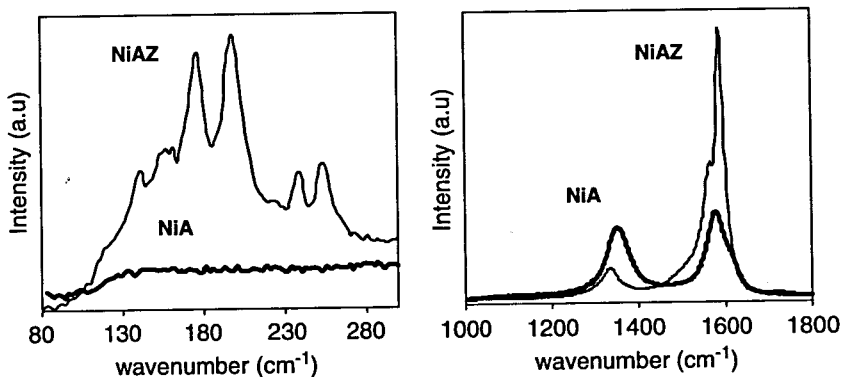
Fig. 6. Raman spectra of carbon species formed after DR deactivation test at 700 °C.
