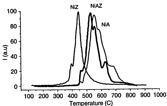
Fig. 2. Temperature programmed reduction TPR profiles for NiZ, NiAZ and NiA catalysts. For the conditions, see the text.
