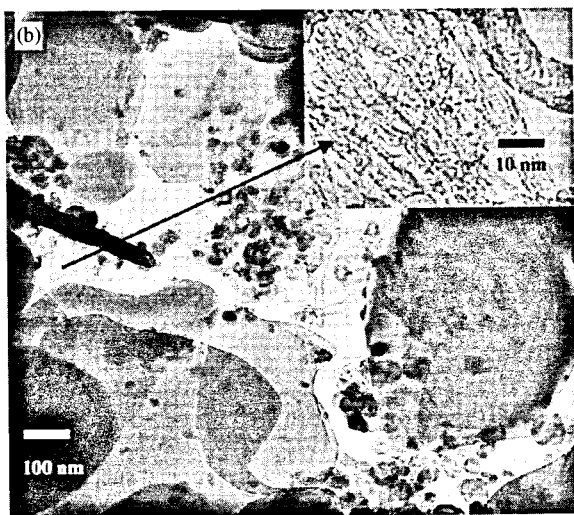
Fig. 4. (a) TEM micrographs of NiA catalyst, after DR deactivation test at 700 °C. (b) TEM micrographs of NiAZ catalyst, after DR deactivation test at 700 °C. The inner figure shows the formation of Single Walled Carbon Nanotubes.
