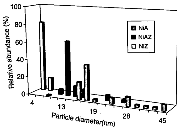
Fig. 1. Particle size distribution for the fresh catalysts (TEM).
