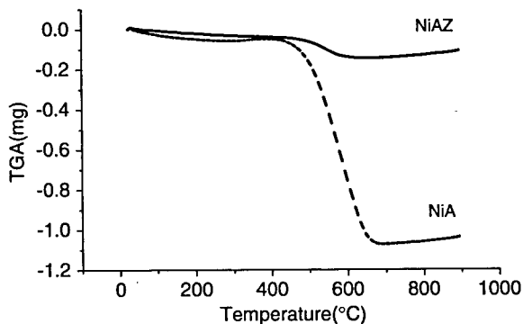
Fig. 5. Temperature-programmed oxidation (TPO) of carbon species formed after DR deactivation test at 700 °C. NiA (---) and NiAZ (—).
