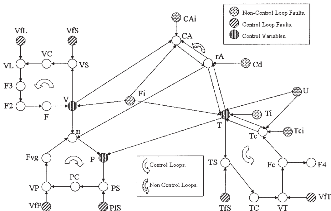
Figure A1. DG diagram of the CSTR.
