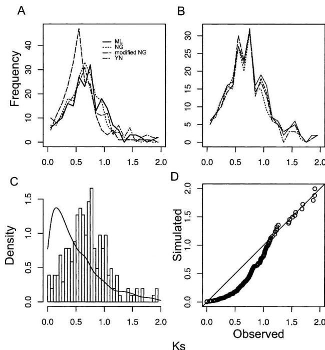
Figure 2. K_s distribution from a sample of Arabidopsis unigenes and the diagnostic test according to the constant birth-death model (null model). (A) K_s estimates from four methods show strong agreement. (ML) Maximum likelihood method by Goldman and Yang; (NG) Nei-Gojobori method; (mNG) modified Nei-Gojobori method; (YN) Yang and Nielsen method. These sample sizes are comparable to the unigenes available for the species sequenced in this study. (B) K_s distributions for paralogs from four replicate unigenes of 6000 sequences each. (C) The density plot of observed K_s distribution and simulated data based on the null model with parameter \delta = 0.67 . (D) The Q-Q plot of observed versus expected K_s values shows the poor fit of the null hypothesis that gene birth and death rates are constant ( P \ll 0.0001 ).
