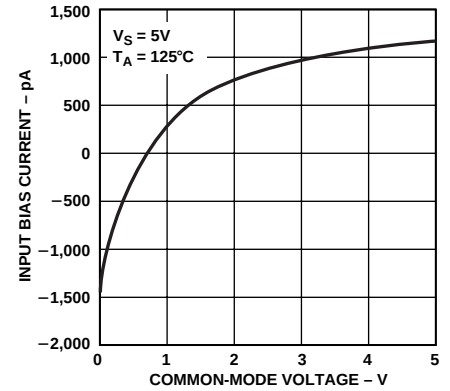
Figure 3. Input Bias Current vs. Common-Mode Voltage
