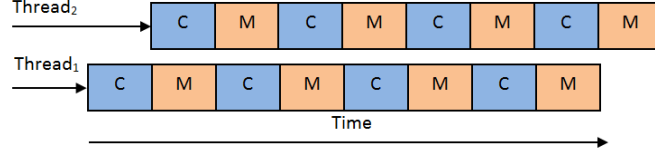
Figure 2.5: Multithreaded execution to hide the effect of memory stalls [13] to reduce access time.
