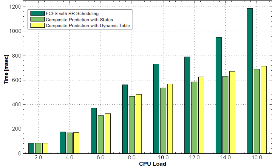
Figure 6.9: Task response time comparison among RR, TASM, and TASE models while the aggregate CPU load, L , was varied from 2.0 – 16.0.
