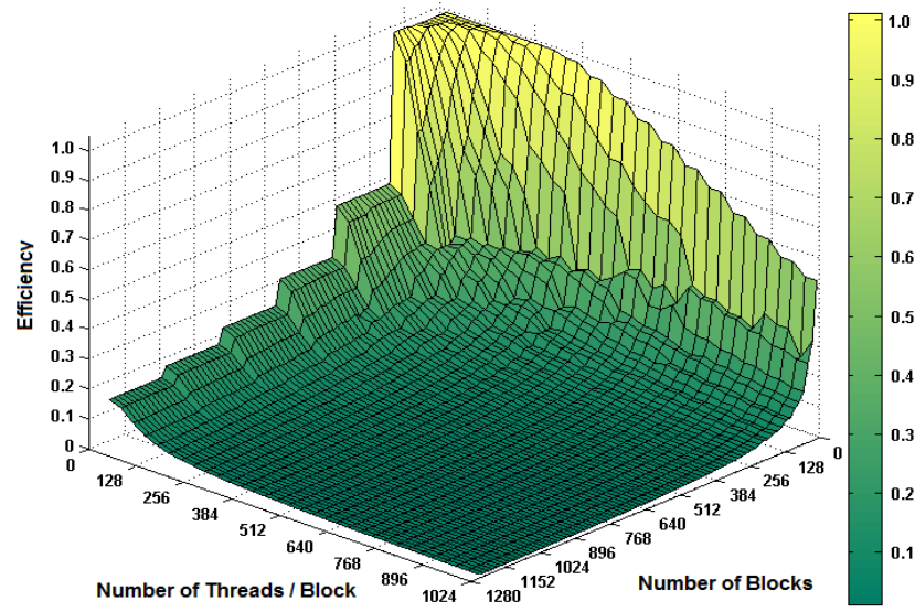
Figure 7.5: Surface diagrams for the Sum of Binomial Series benchmark program (a) Surface diagram shows increasing run-time while \vartheta increased from 32 to 1248 and \beta increased from 16 to 1024 (b) The measured efficiency surface diagram with respect to the ideal execution time ( \tau ).
