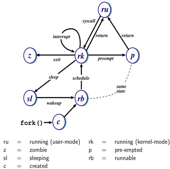
Figure 2.1: Various states of Unix Processes [34].
