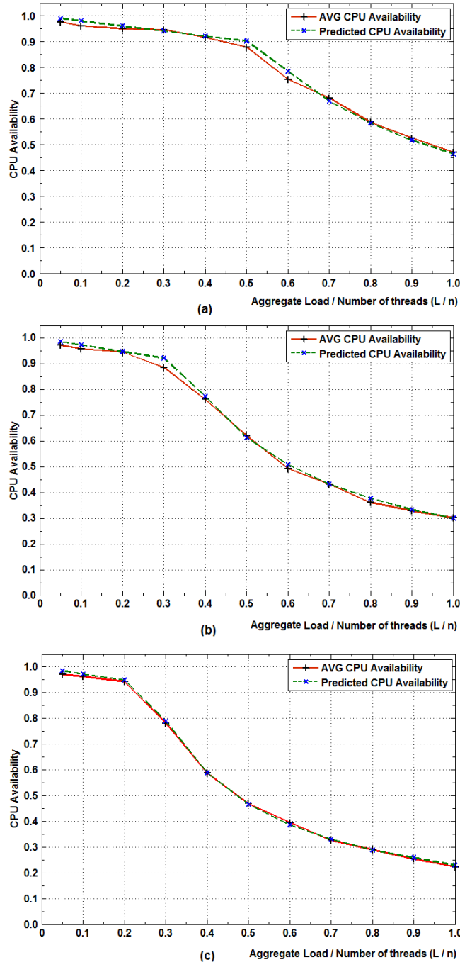
Figure 4.8: The measured average CPU availability data (first set) and predicted average data associated with Eq. 4.6 for (a) Multi-core systems with r = 4 and n = 8 . (b) Multi-core systems with r = 4 and n = 12 . (c) Multi-core systems with r = 4 and n = 16 .
