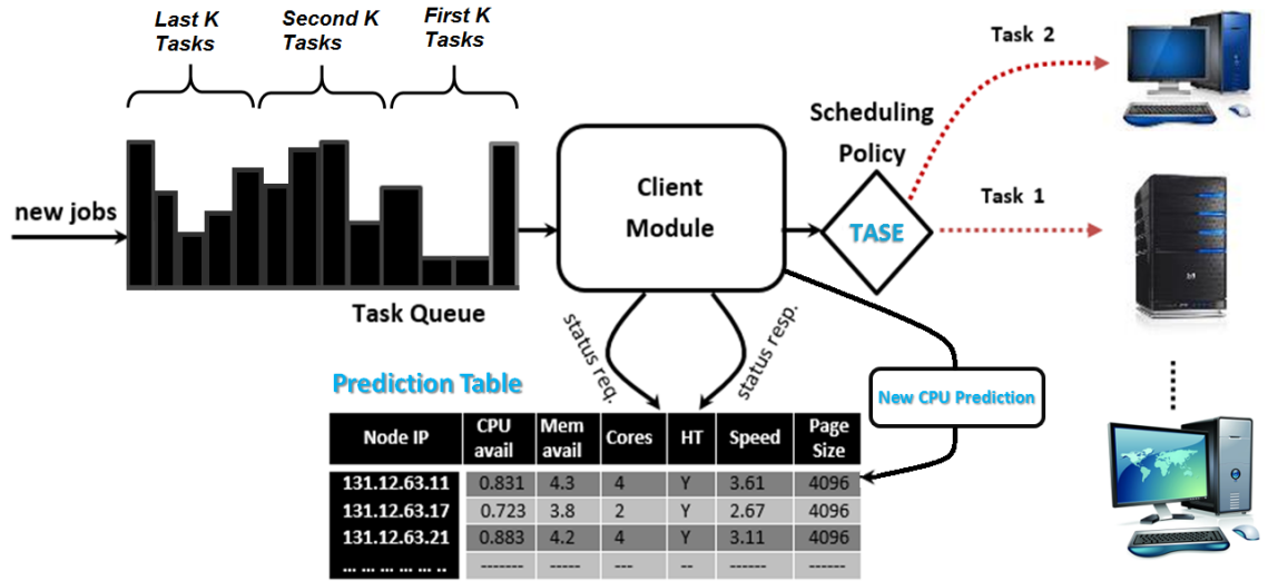
Figure 6.3: Task assignment to distributed compute nodes using a dynamic prediction table consists of real-time prediction of status data of compute nodes.
