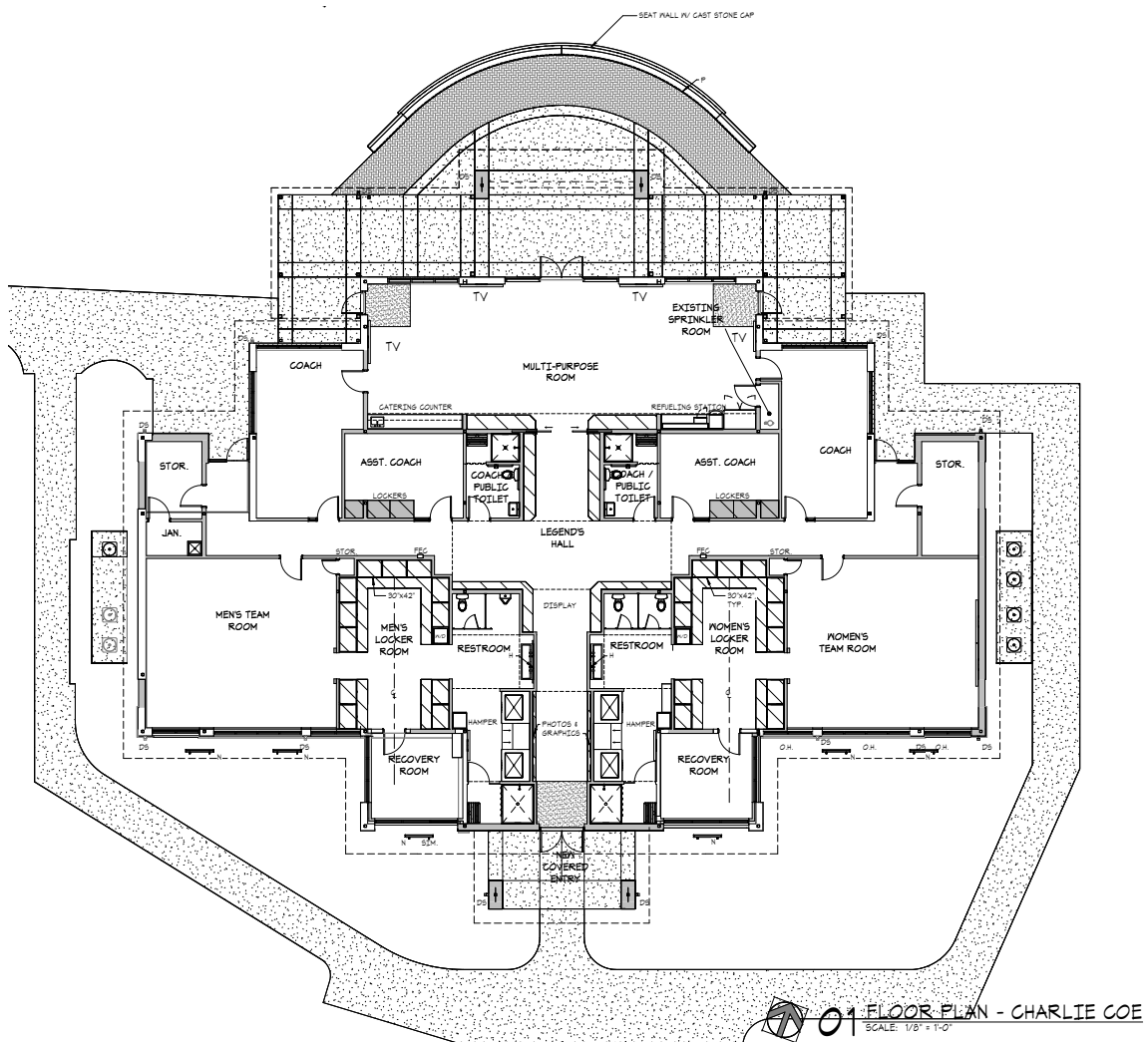
CHARLIE COE GOLF LEARNING CENTER RENOVATION - FLOOR PLAN
